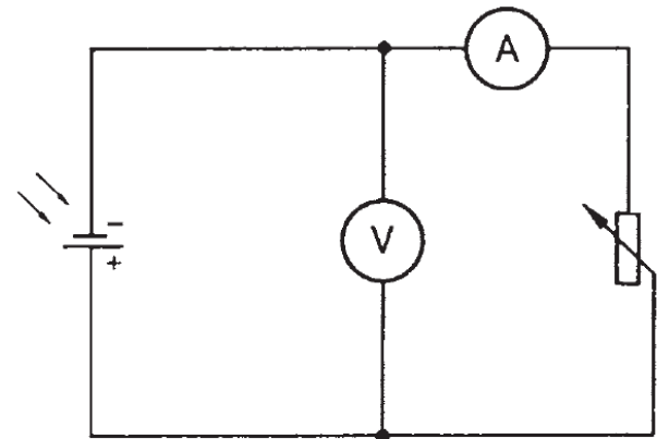
Fig. 2: Circuit for measuring the current-voltage characteristic.
