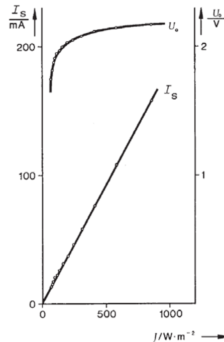
Fig. 6: Short-circuit current I_s and no-load voltage U_0 as a function of the light intensity J .
