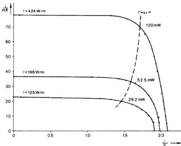
Fig. 7: Current-voltage characteristic at different light intensities J .
