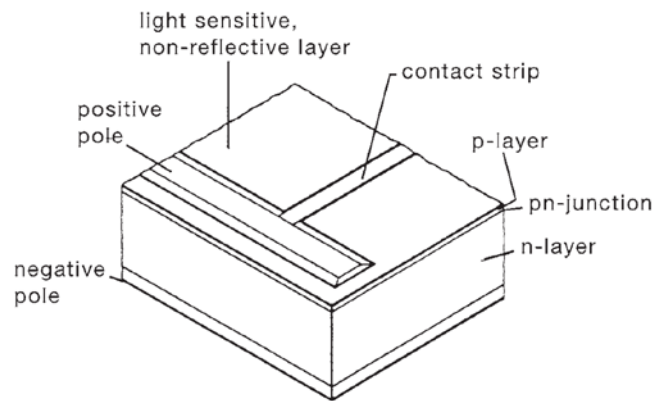
Fig. 4: Construction of a silicon solar cell.
