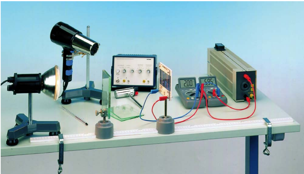
Fig. 1: Set-up of experiment P2410901
